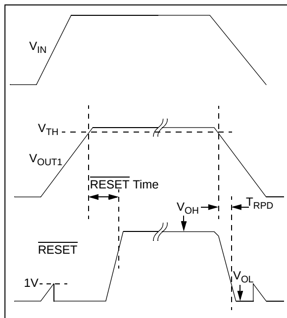
FIGURE 5-4: TC1301B RESET Timing.
