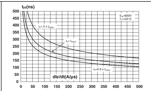
Figure 6. Reverse recovery time versus dl_F/dt (typical values)
