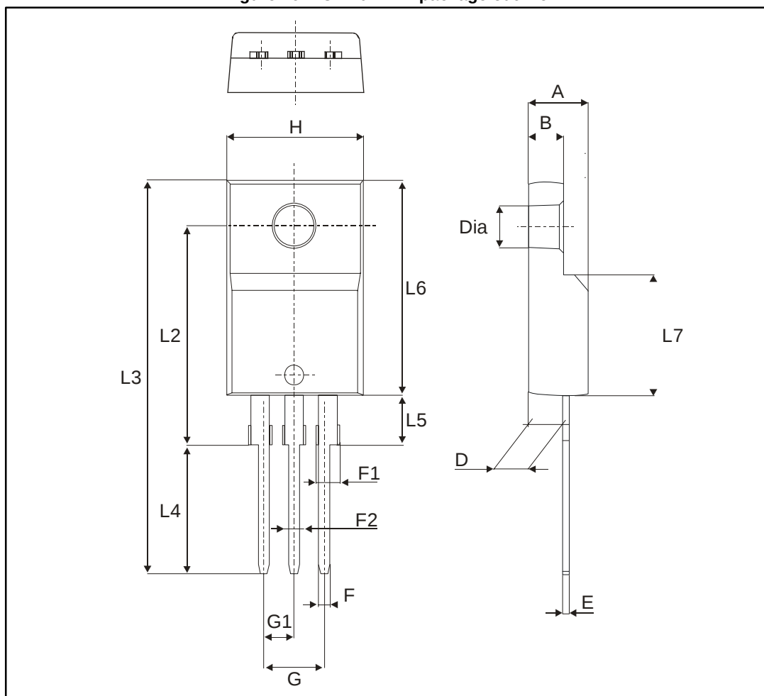
Figure 16: TO-220FPAB package outline
