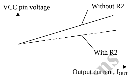
Figure 10-2 Variation of VCC pin voltage and power
