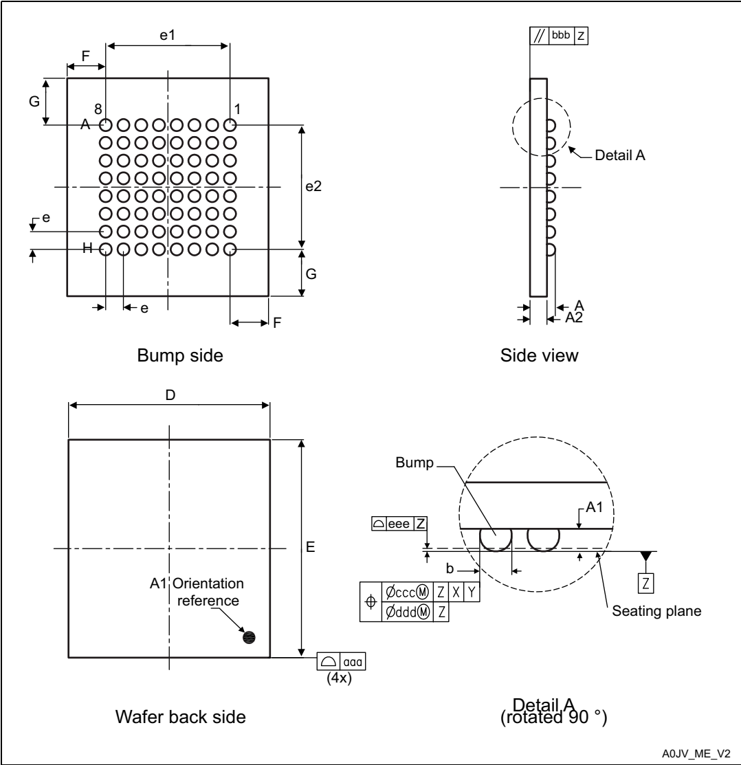
Figure 43. WLCSP64 outline
