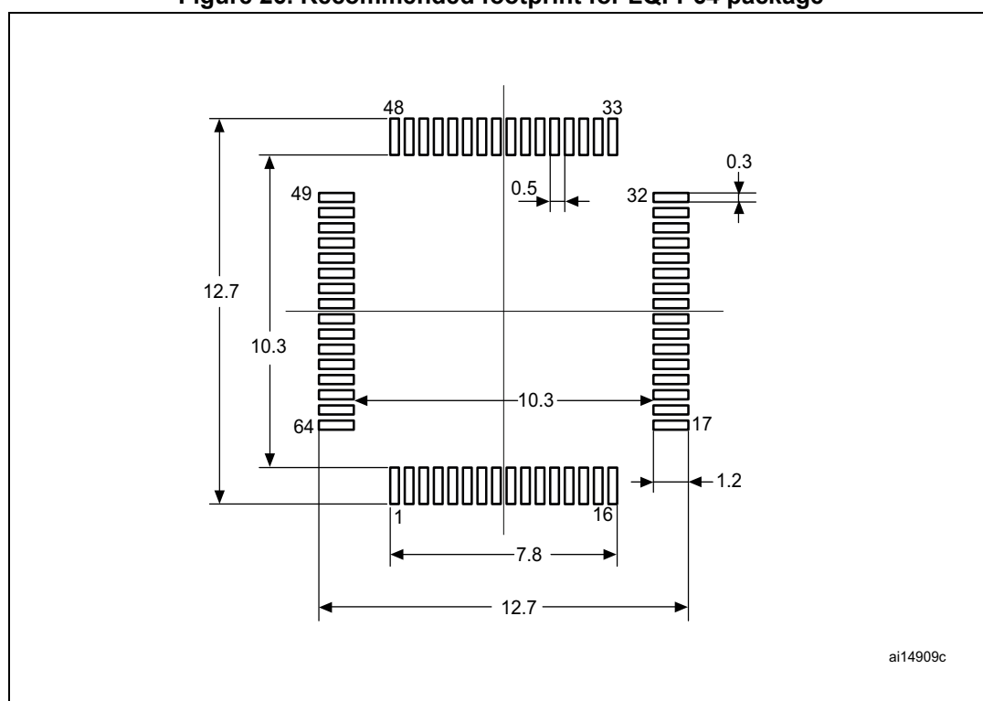
Figure 26. Recommended footprint for LQFP64 package
