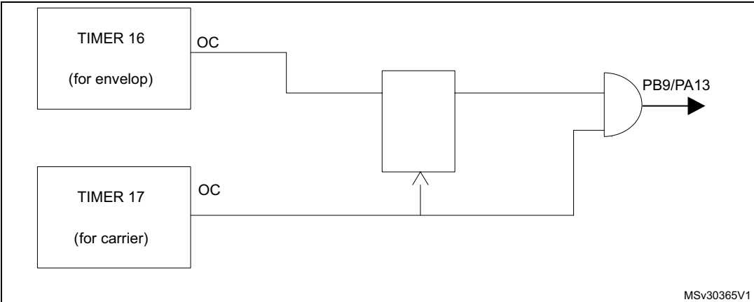
Figure 3. Infrared transmitter
