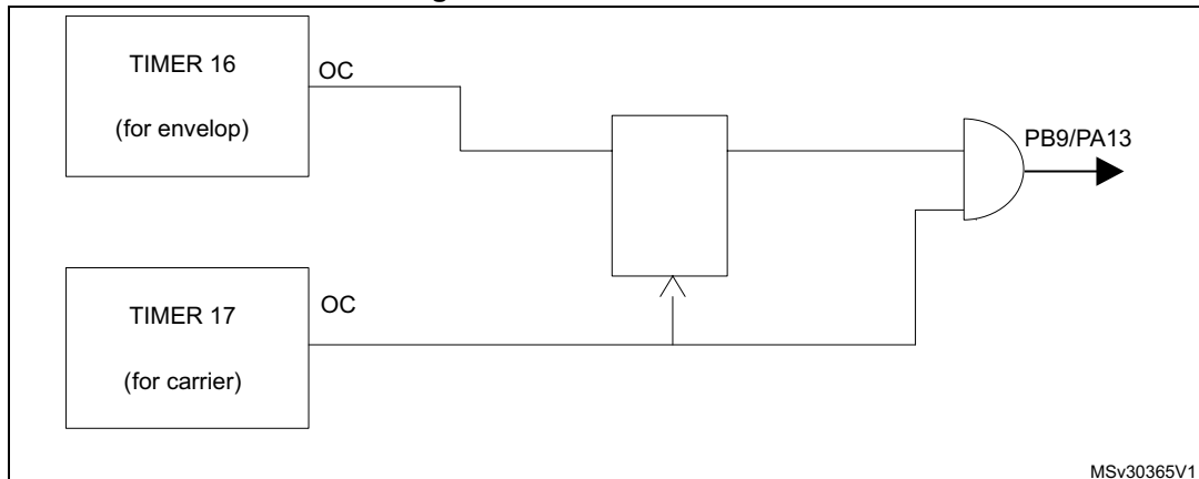
Figure 3. Infrared transmitter
