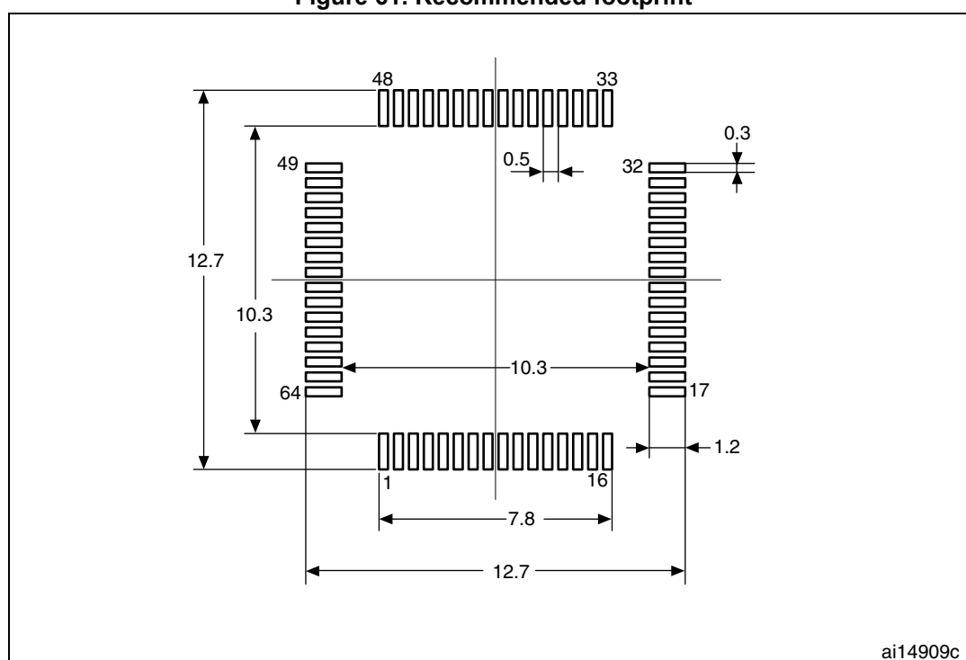
Figure 61. Recommended footprint
