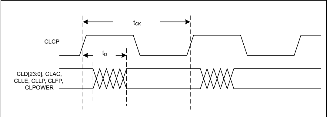
Figure 9. CLCD waveform
