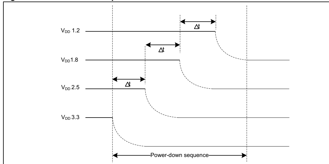
Figure 5. Power-down sequence
