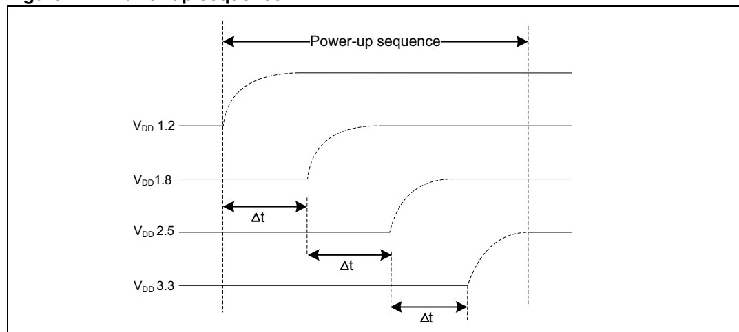
Figure 4. Power-up sequence
