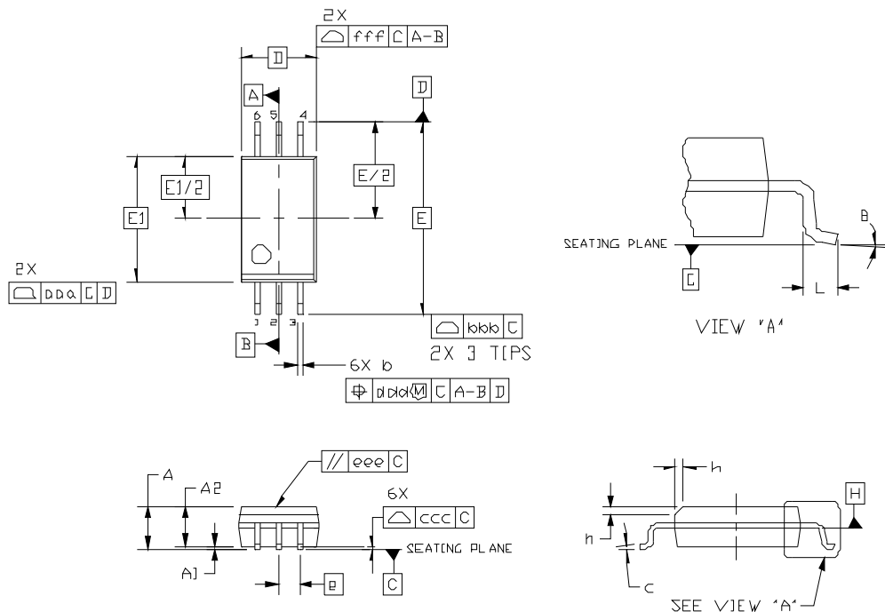
Figure 20. SDIP6 Package
