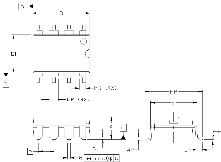
Figure 18. DIP8 Package
