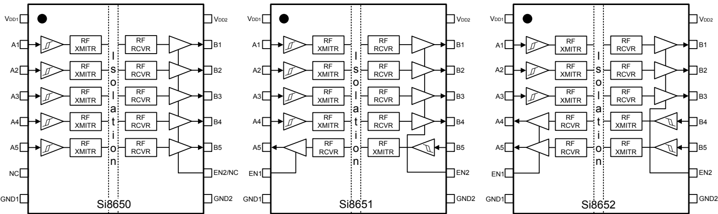
Figure 5.1. Si8650/51/52 Pinout
