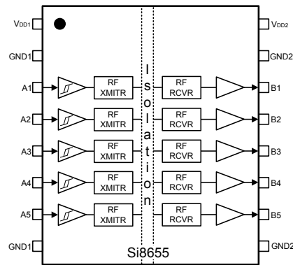
Figure 5.2. Si8655 Pinout
