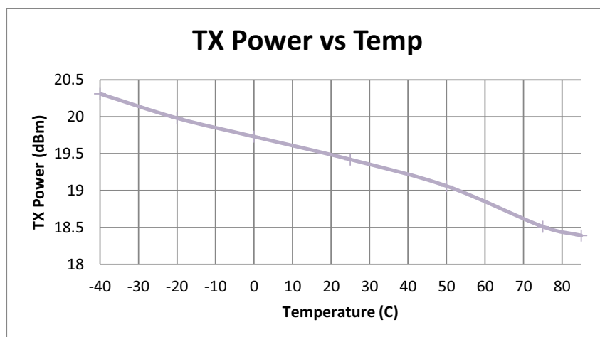
Figure 9. +20 dBm TX Power vs. Temp
