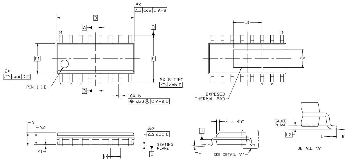
Figure 37. 16-Pin Thermal Enhanced Small Outline Integrated Circuit (ESOIC) Package
