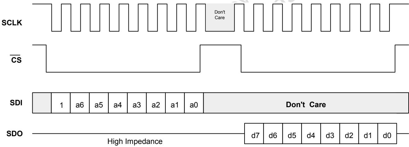
Figure 27. Serial Read 8-Bit Mode
