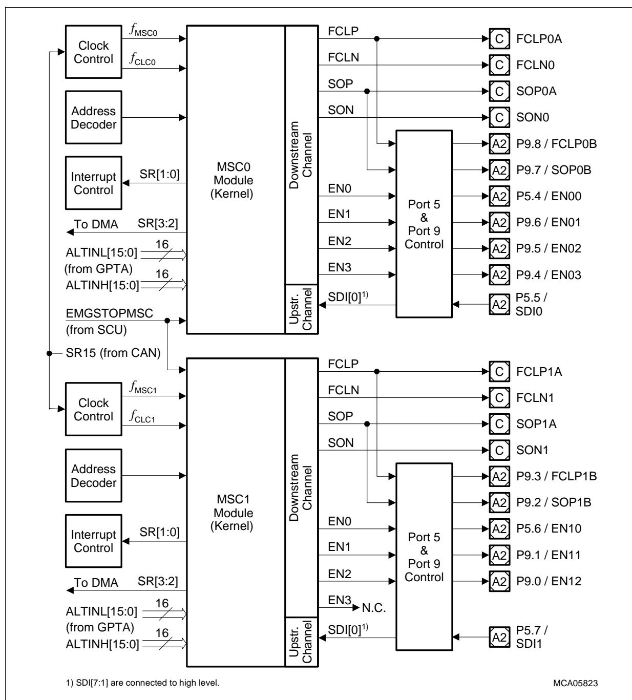
Figure 10 Block Diagram of the MSC Interfaces
