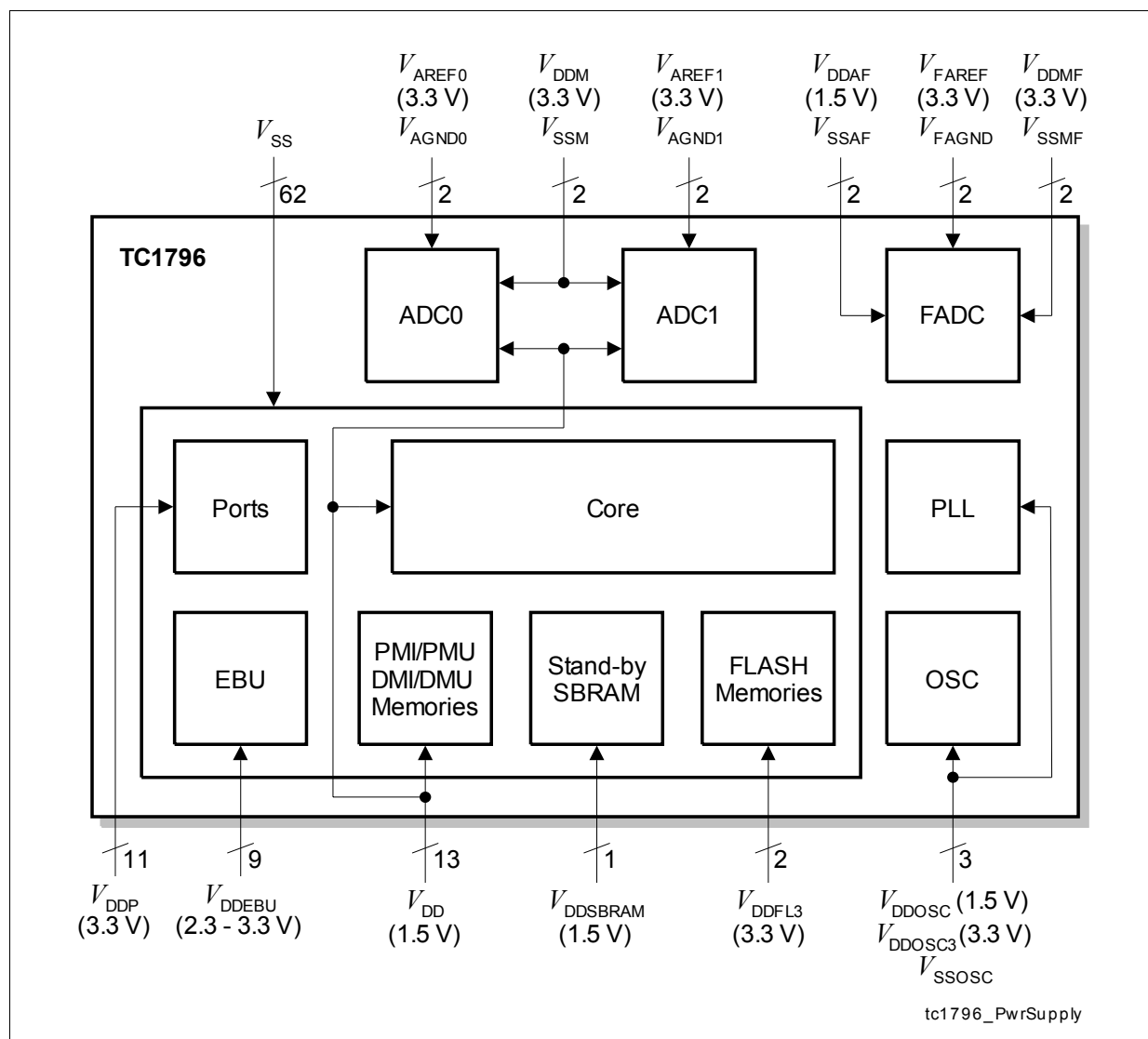
Figure 21 Power Supply Concept of TC1796
