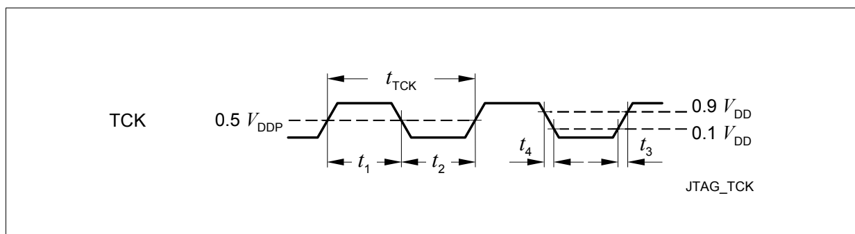
Figure 36 TCK Clock Timing
