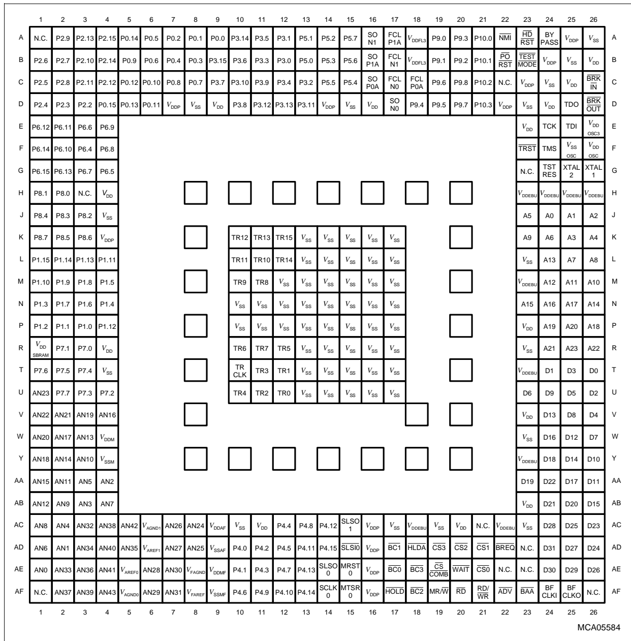
Figure 3 TC1796 Pinning for P/PG-BGA-416-4 Package (Top view)
