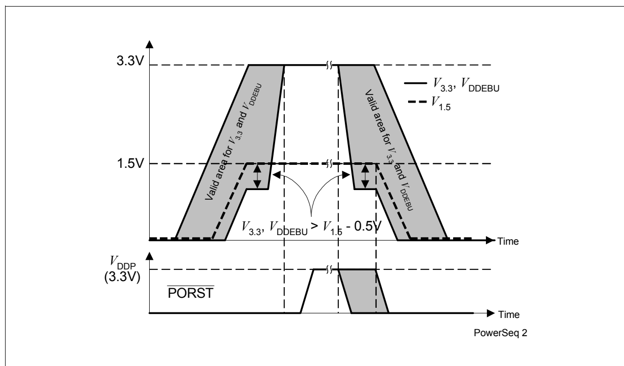
Figure 29 V_{DDP} / V_{DDEBU} / V_{DD} Power Up Sequence
