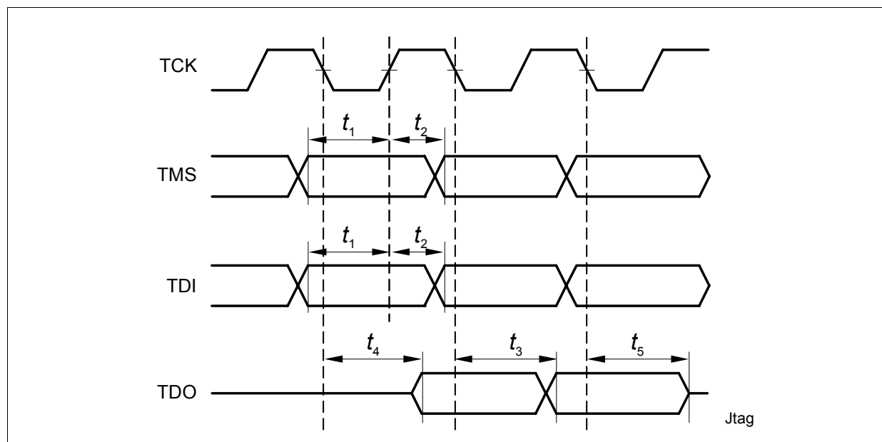
Figure 37 JTAG Timing
