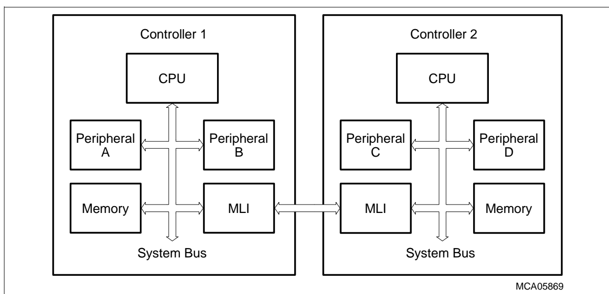
Figure 12 Typical Micro Link Interface Connection
