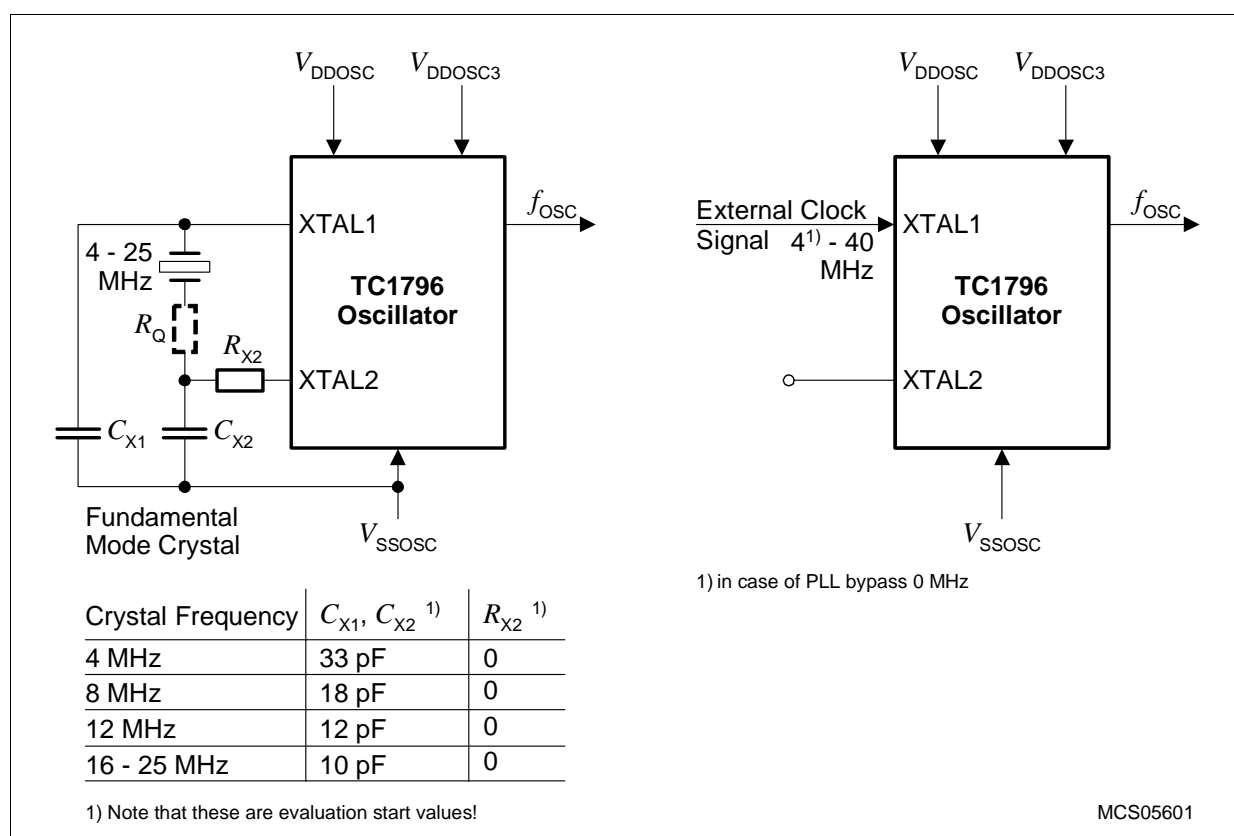
Figure 20 Oscillator Circuitries
