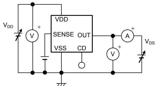
Figure 10 Test Circuit 3
