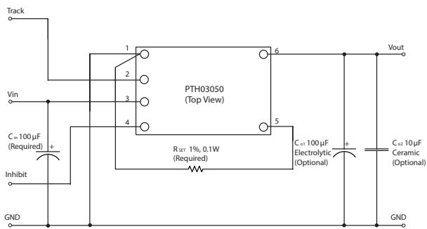
Figure 3 - Standard Application
