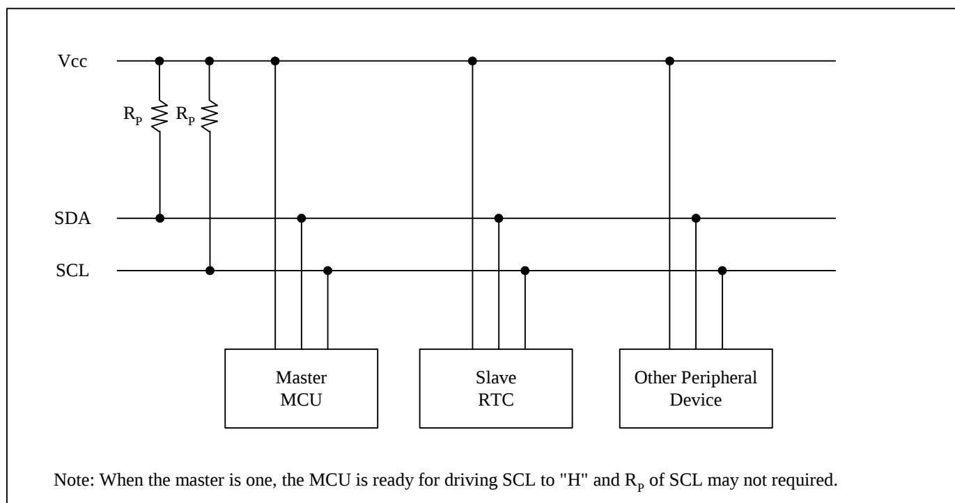
Fig 4. System configuration
