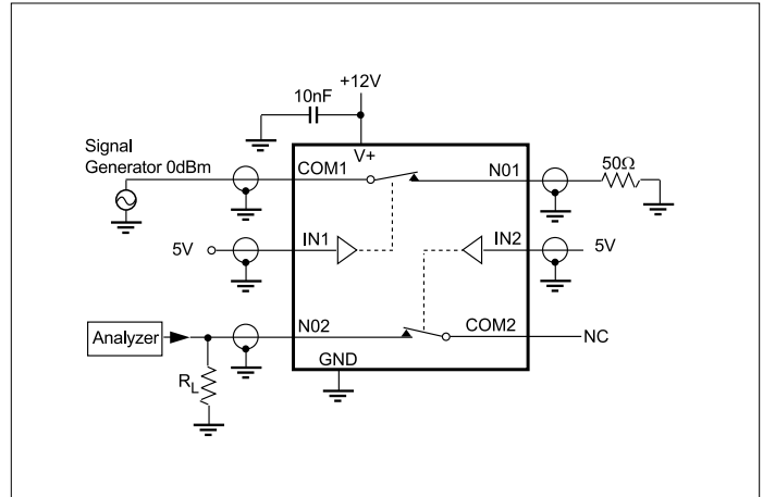
Figure 5. Crosstalk
