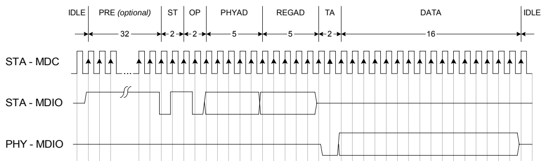
Figure 31 MDC/MDIO Read Cycle
