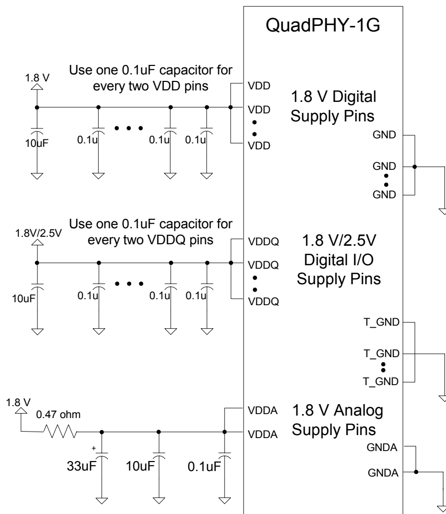
Figure 33 Recommended Power Supply Decoupling
