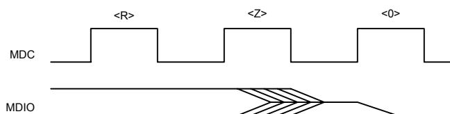
Figure 32 Behavior of MDIO During TA Field of a Read Transaction
