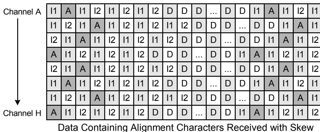
Figure 15 Trunking Mode Channel Alignment using Alignment Characters
