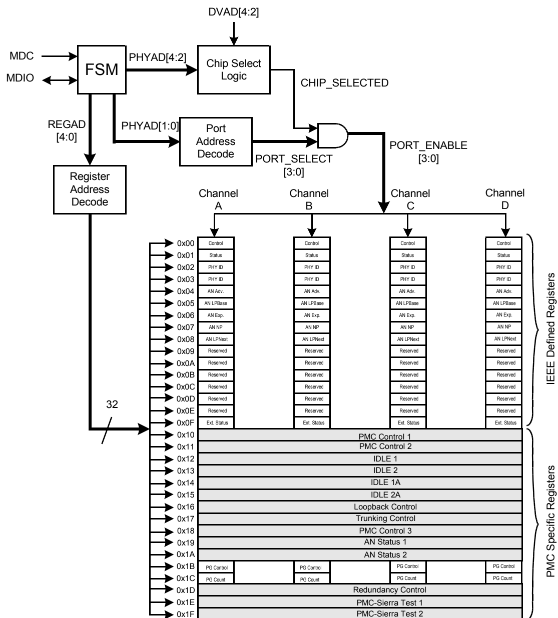
Figure 25 Register Access
