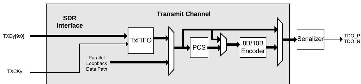
Figure 10 Transmit Channel Functional Blocks
