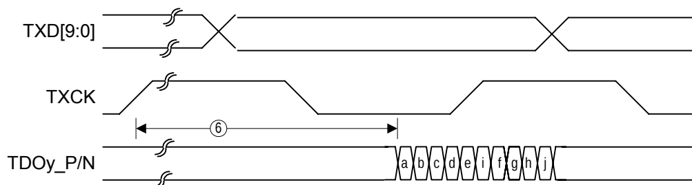
Figure 42 Transmit Latency
