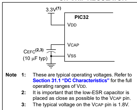
FIGURE 28-1: CONNECTIONS FOR THE ON-CHIP REGULATOR
