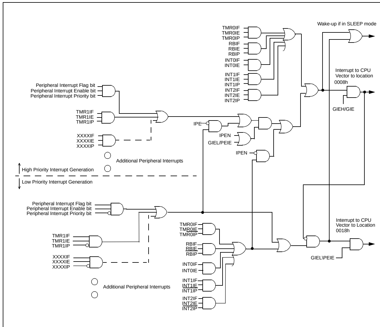
FIGURE 7-1: INTERRUPT LOGIC
