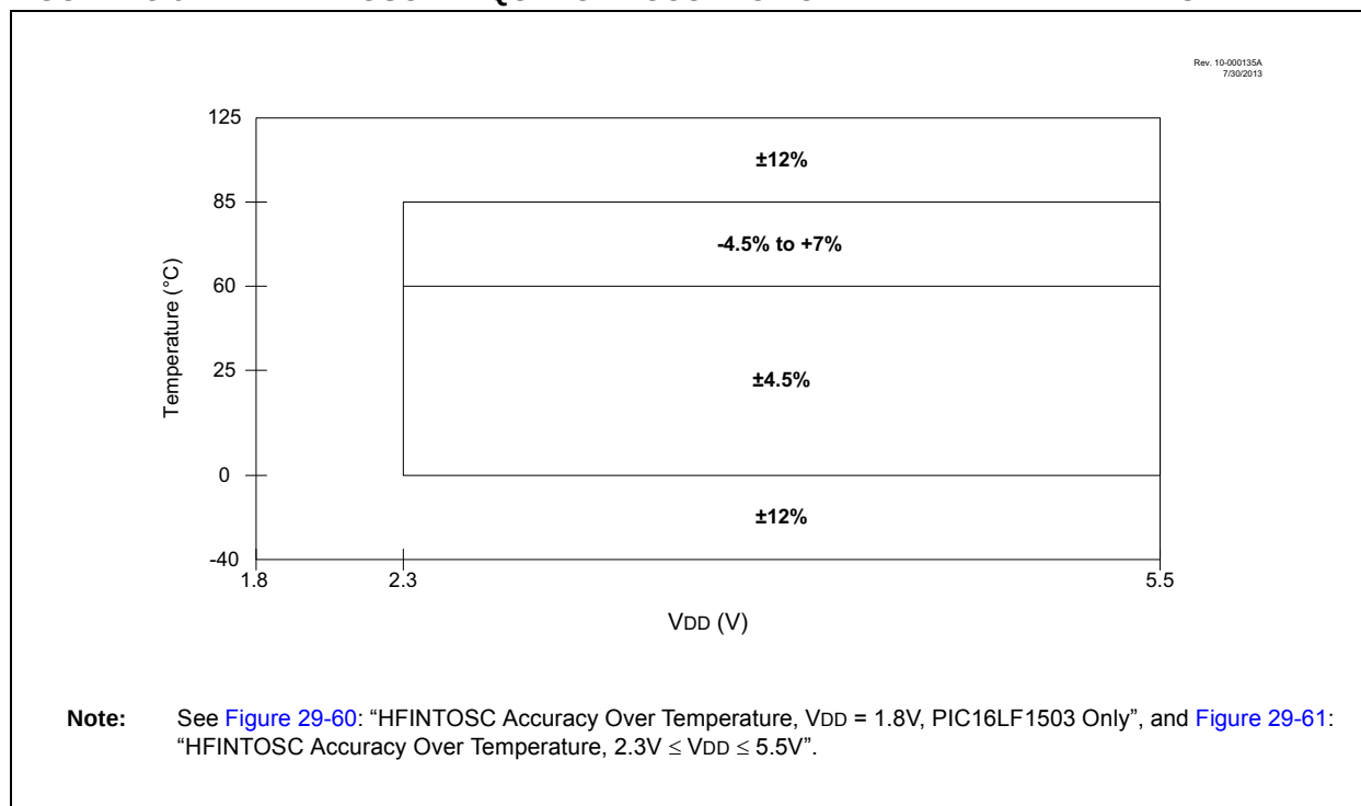
FIGURE 28-6: HFINTOSC FREQUENCY ACCURACY OVER V DD AND TEMPERATURE
