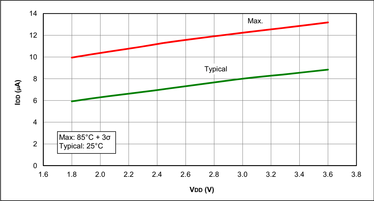
FIGURE 29-1: I_{DD} , EXTERNAL CLOCK (ECL), LOW-POWER MODE, F_{osc} = 32\text{ kHz} , PIC16LF1503 ONLY
