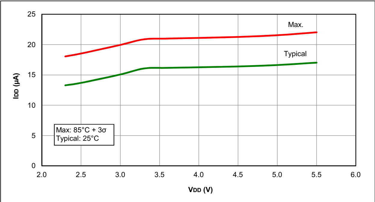
FIGURE 29-2: I_{DD} , EXTERNAL CLOCK (ECL), LOW-POWER MODE, F_{osc} = 32\text{ kHz} , PIC16F1503 ONLY
