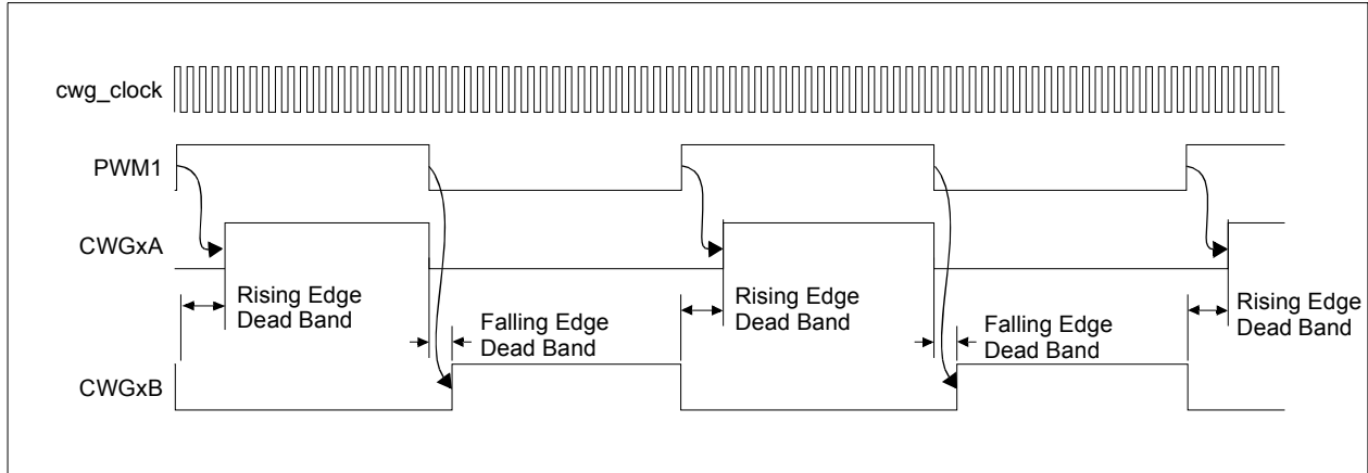
FIGURE 22-2: TYPICAL CWG OPERATION WITH PWM1 (NO AUTO-SHUTDOWN)
