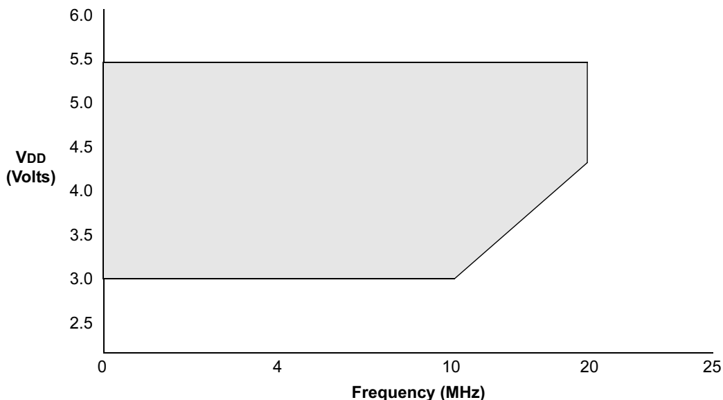
FIGURE 10-1: PIC16LC554/557/558 VOLTAGE-FREQUENCY GRAPH, 0^{\circ}\text{C} \leq T_A \leq +70^{\circ}\text{C} (COMMERCIAL TEMPS)
