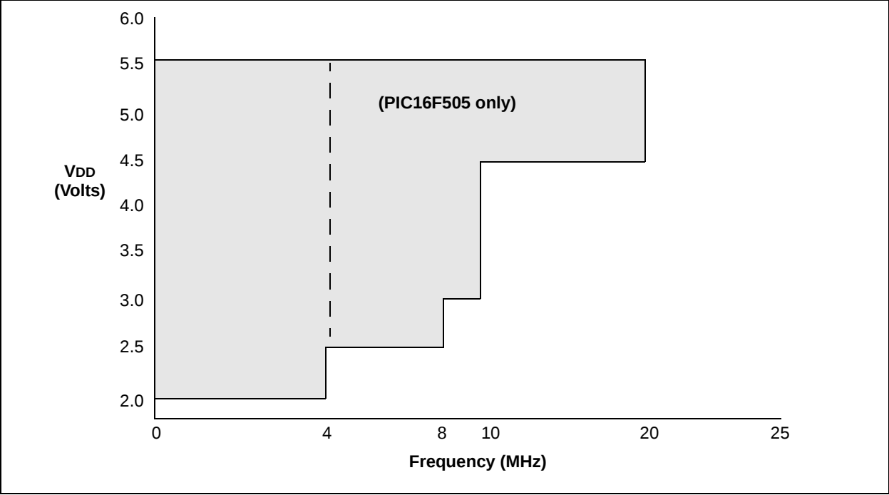
FIGURE 10-1: PIC12F508/509/16F505 VOLTAGE-FREQUENCY GRAPH, -40°C ≤ TA ≤ +125°C
