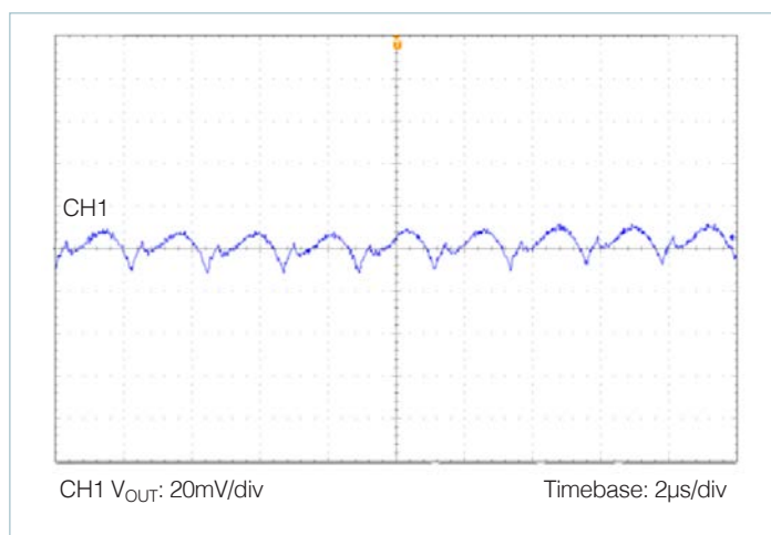
Figure 23 — Output voltage ripple: nominal line, nominal trim, 50% load, C_{OUT} = 8 \times 100\mu\text{F} ceramic
