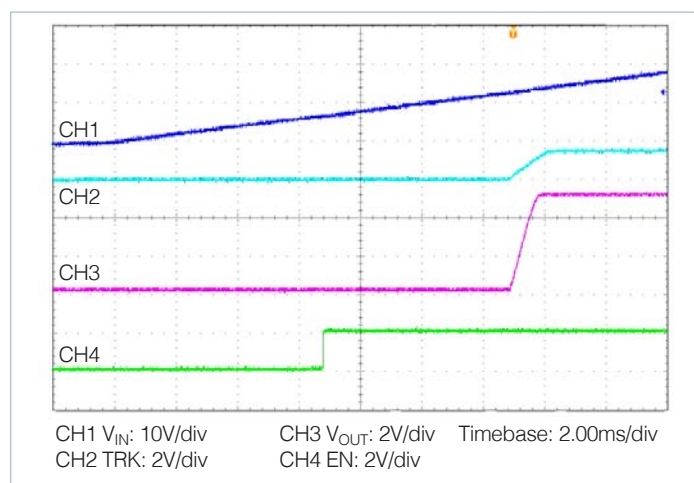
Figure 56 — Start up from V_{IN} applied, nominal line, nominal trim, typical timing, PI3325 shown
