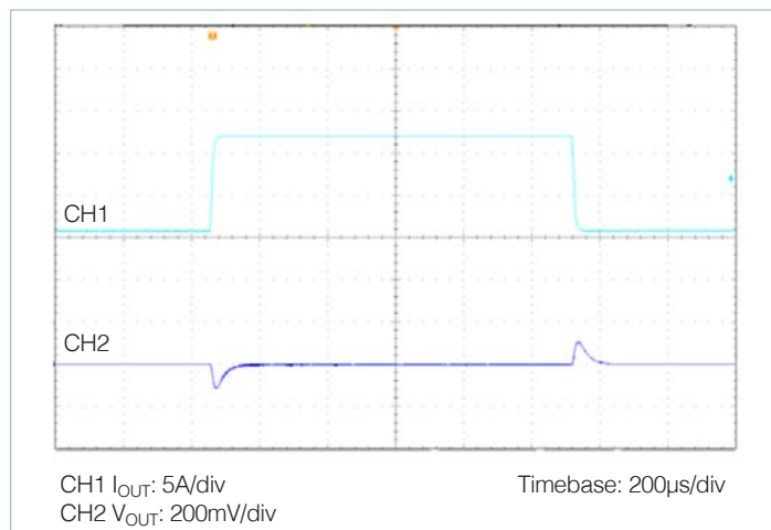
Figure 19 — Transient response: 50 – 100% load, at 1A/µs. nominal line, nominal trim, C_{OUT} = 8 \times 100\mu\text{F} ceramic
