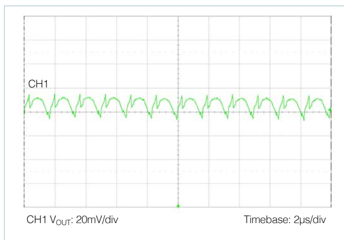
Figure 51 — Output voltage ripple: nominal line, nominal trim, 50% load, C_{OUT} = 12 \times 47\mu F ceramic
