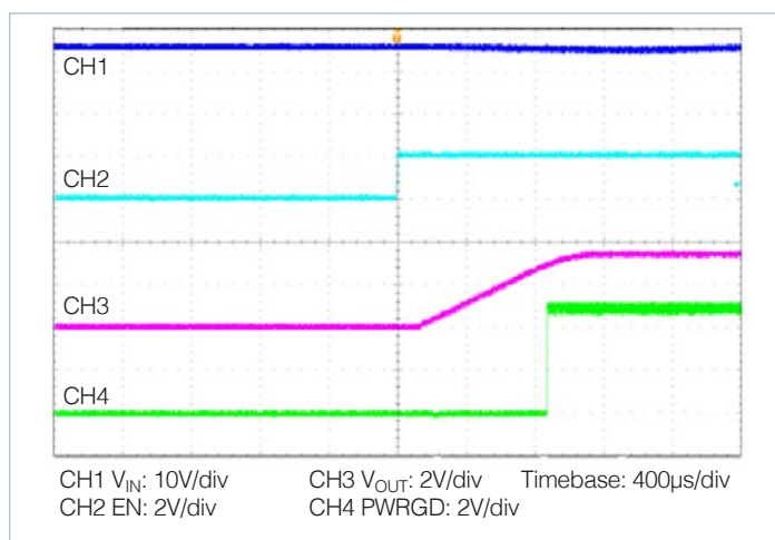
Figure 28 — Start up from EN, V_{IN} pre-applied, nominal line, nominal trim, typical timing, PI3323 shown
