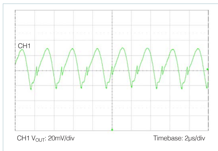
Figure 48 — Output voltage ripple: nominal line, nominal trim, 100% load, C_{OUT} = 12 \times 47\mu F ceramic
