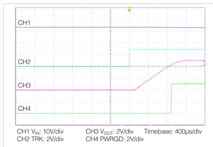
Figure 57 — Start up from EN, V_{IN} pre-applied, nominal line, nominal trim, typical timing, PI3325 shown
