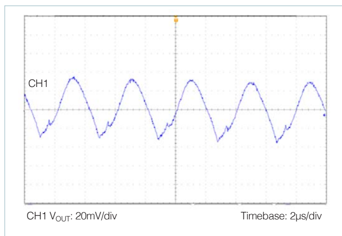
Figure 20 — Output voltage ripple: nominal line, nominal trim, 100% load, C_{OUT} = 8 \times 100\mu\text{F} ceramic
