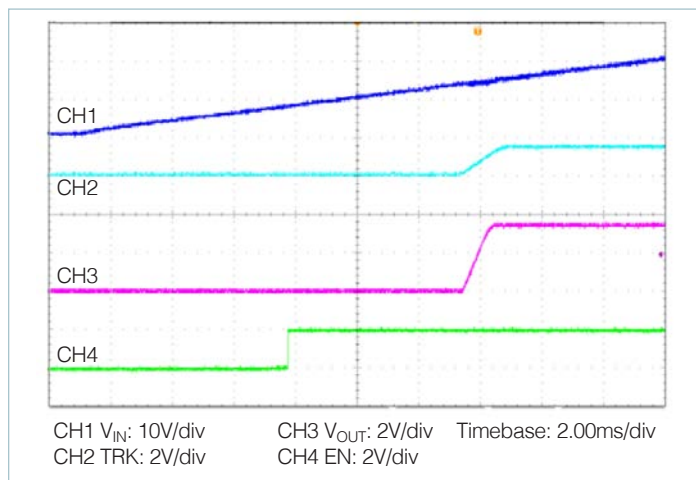
Figure 27 — Start up from V_{IN} applied, nominal line, nominal trim, typical timing, PI3323 shown
