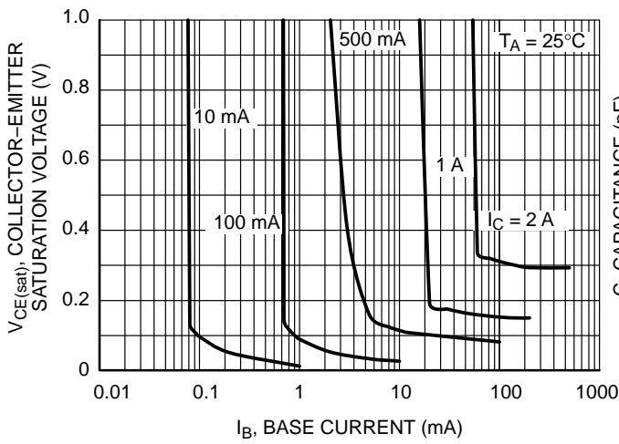
Figure 6. Saturation Region
