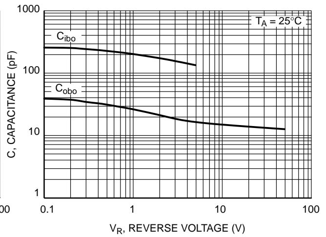
Figure 7. Capacitance
