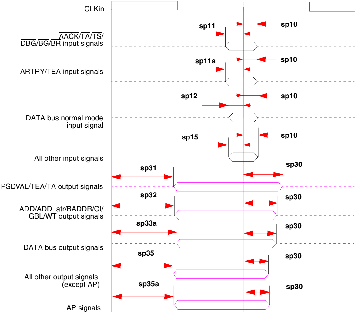
Figure 9. Bus Signals
