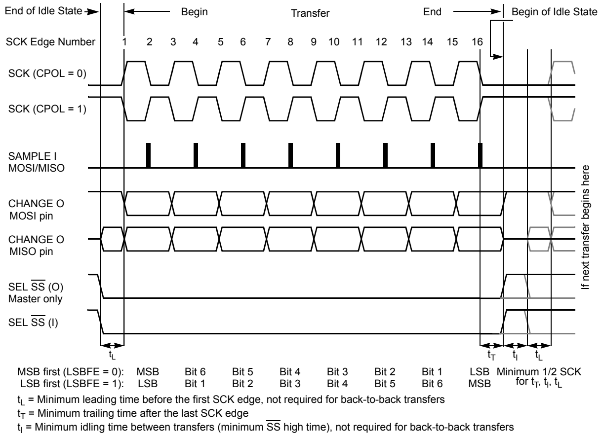
Figure 104. SPI Clock Format 1 (CPHA = 1), with 8-Bit Transfer Width Selected (XFRW = 0)
