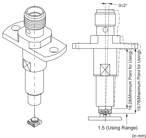
Fig. 1 Insertion the Automatic Measurement Probe (MM126036) in Receptacle (MM8130-2600)
