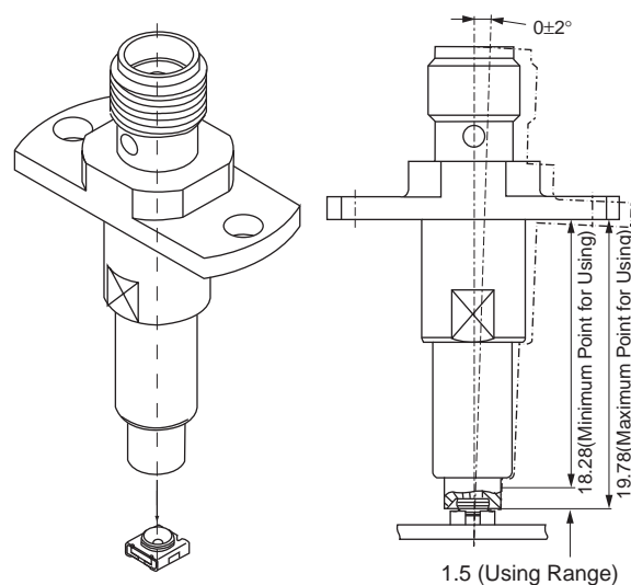
Fig. 1 Insertion the Automatic Measurement Probe (MM126036) in Receptacle (MM8430-2610)
