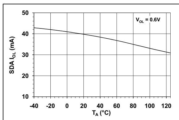
FIGURE 2-9: SDA I_{OL} Vs. Temperature.
