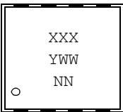
8-Lead 2x3 mm DFN (MCP6031 and MCP6033)
