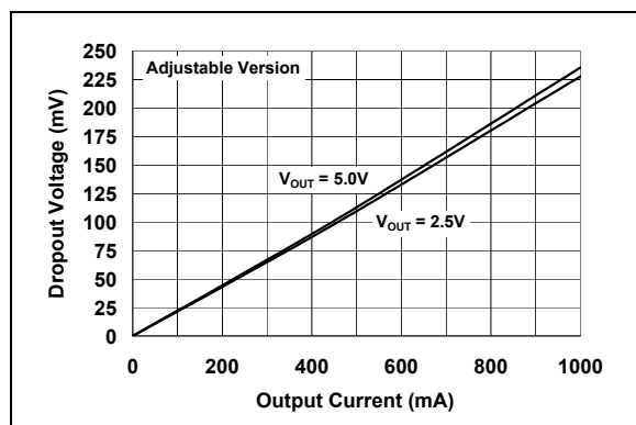
FIGURE 2-7: Dropout Voltage vs. Output Current (Adjustable Version).
