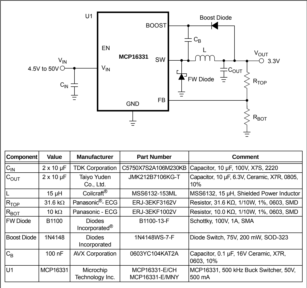
FIGURE 6-1: Typical Application, 50V V IN to 3.3V V OUT .
