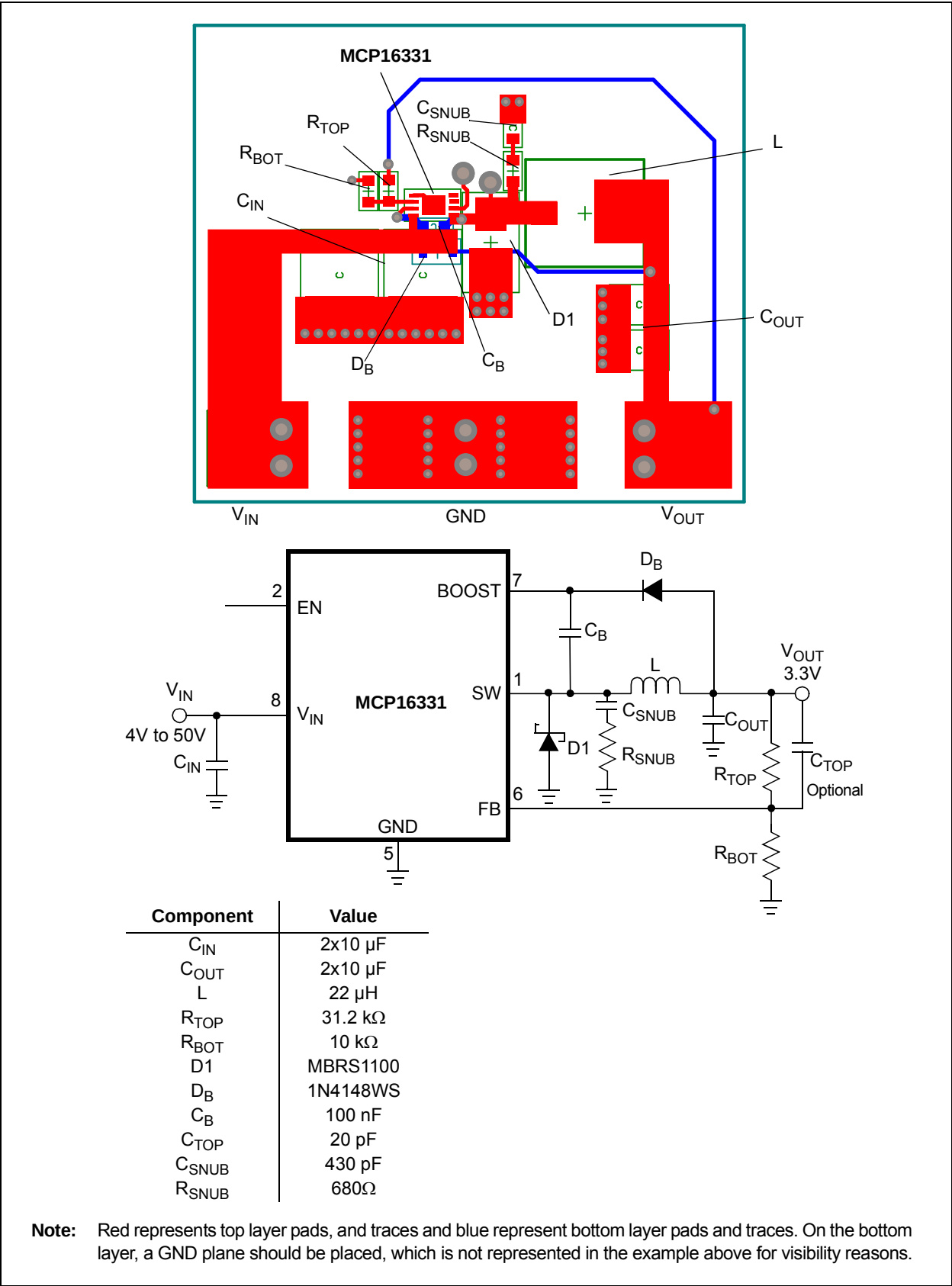
FIGURE 5-3: MCP16331 TDFN-8 Recommended Layout Design.
