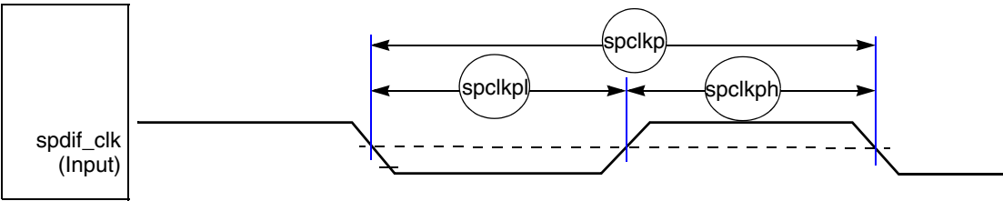
Figure 35. spdif_clk Timing
