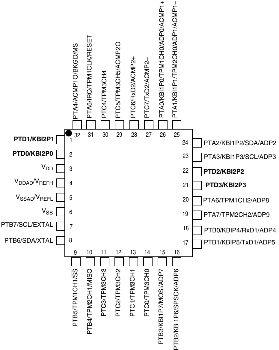
Figure 4. 32-Pin LQFP/QFN
