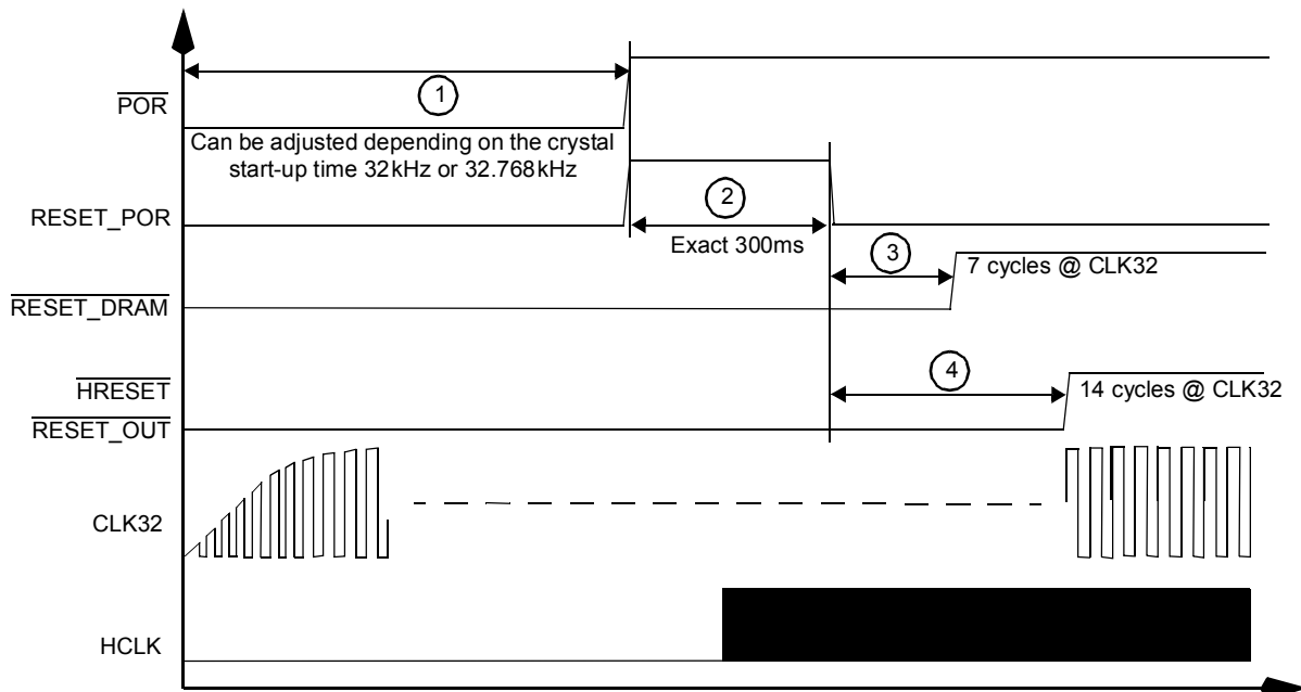
Figure 2. Timing Relationship with \overline{POR}
