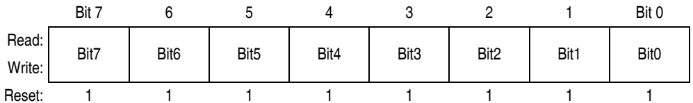
Figure 14-8. TIM Counter Modulo Low Register (TMODL)
