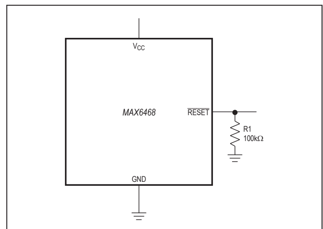
Figure 3. \overline{RESET} Valid to V_{CC} = 0V
