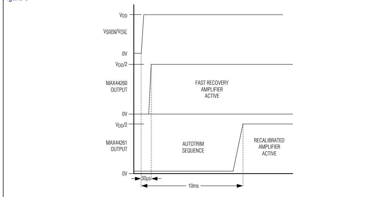
Figure 3. CAL vs. SHDN Input Operation
