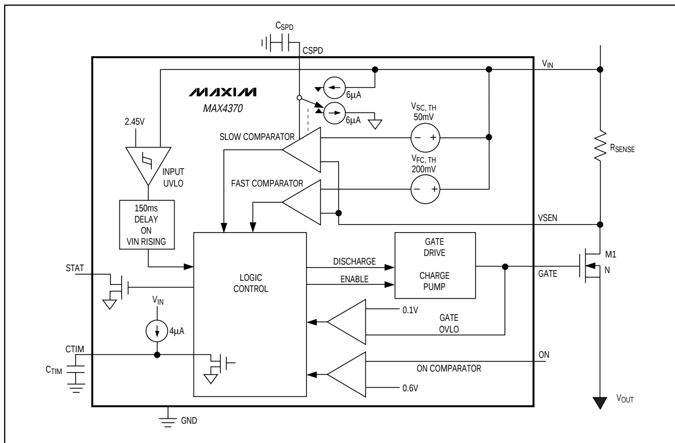
Figure 1. Functional Diagram
