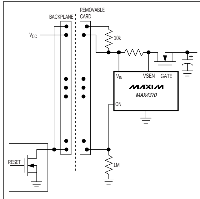
Figure 10. Fail-Safe Connector
