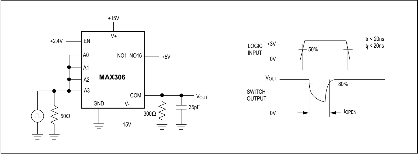
Figure 4. Break-Before-Make Interval
