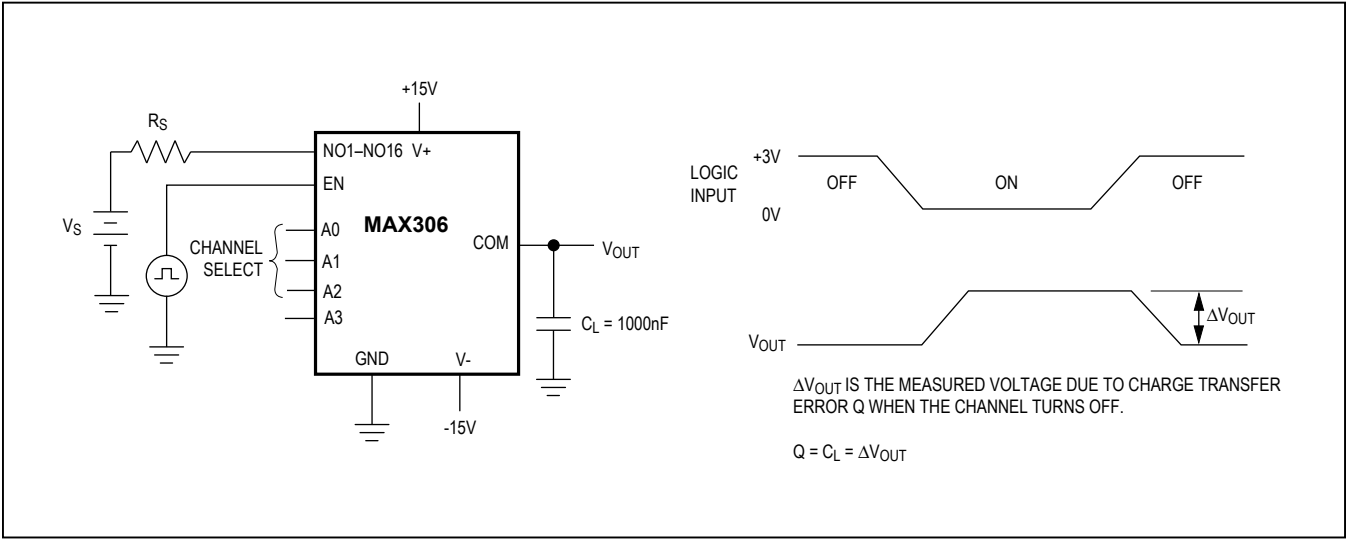
Figure 5. Charge Injection
