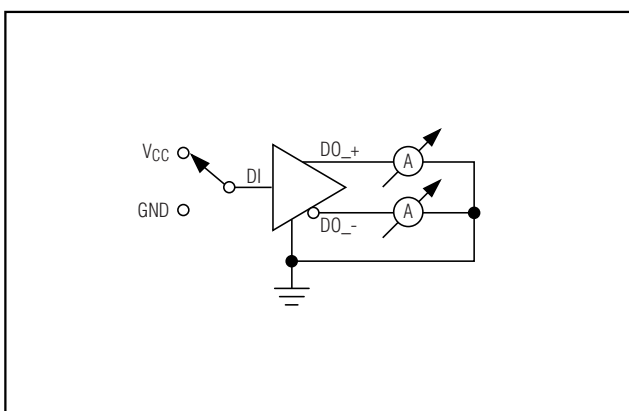
Figure 6. Short-Circuit Measurements
