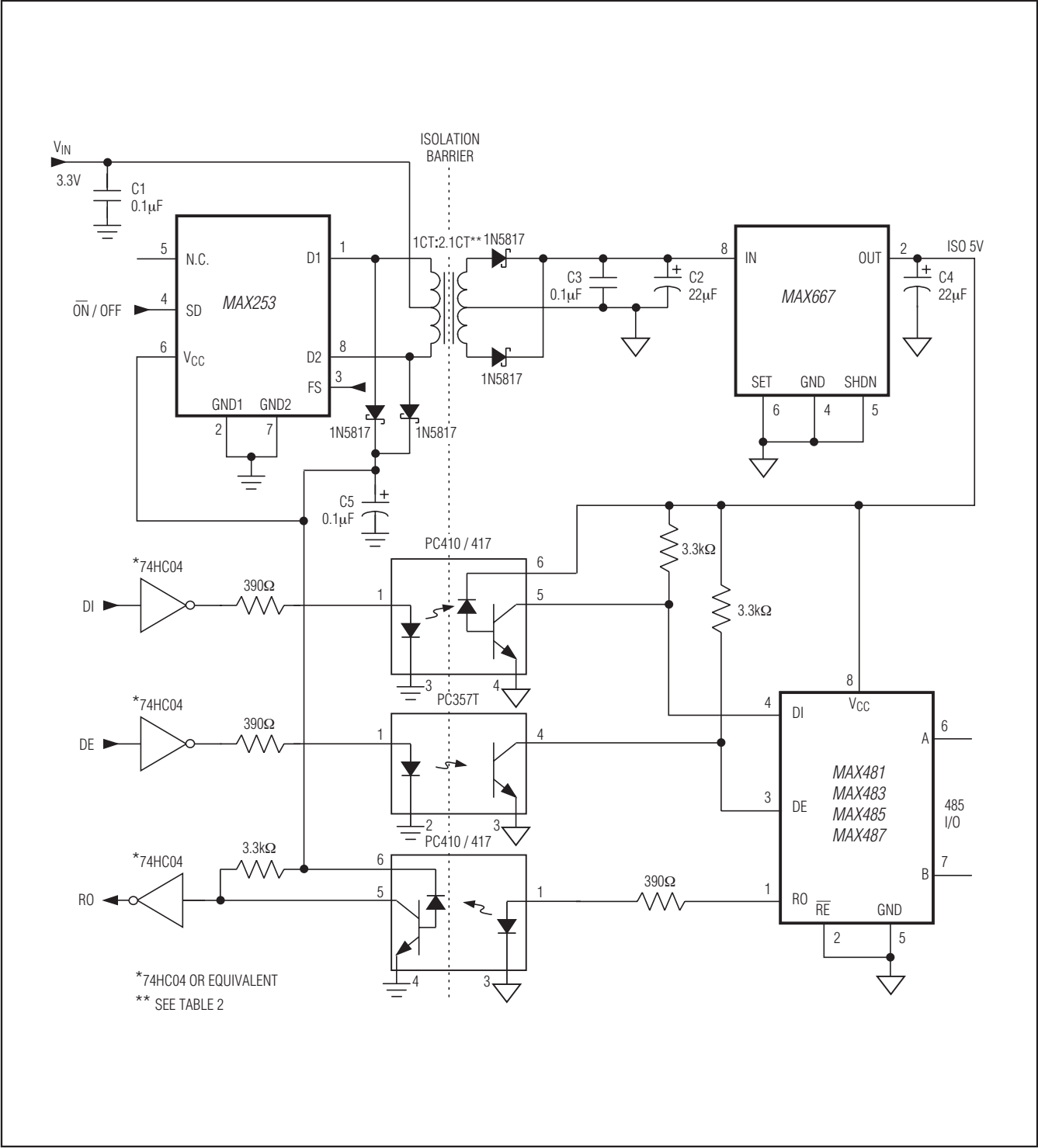
Figure 4. Typical RS-485 Application Circuit, 3.3V Configuration
