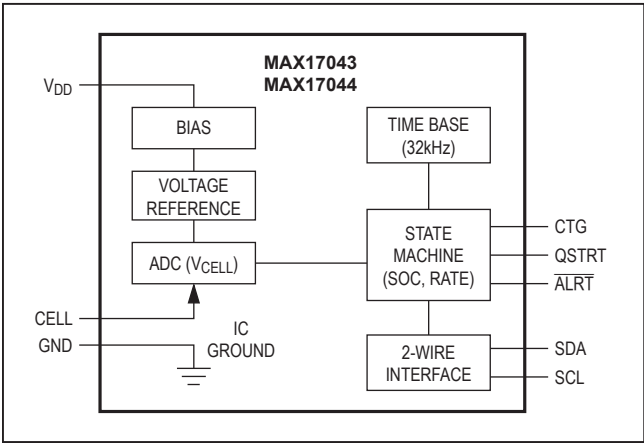
Figure 2. Block Diagram
