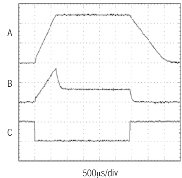
MAX1626 SHUTDOWN RESPONSE TIME AND SUPPLY CURRENT
