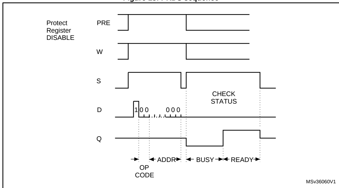
Figure 13: PRDS sequence
