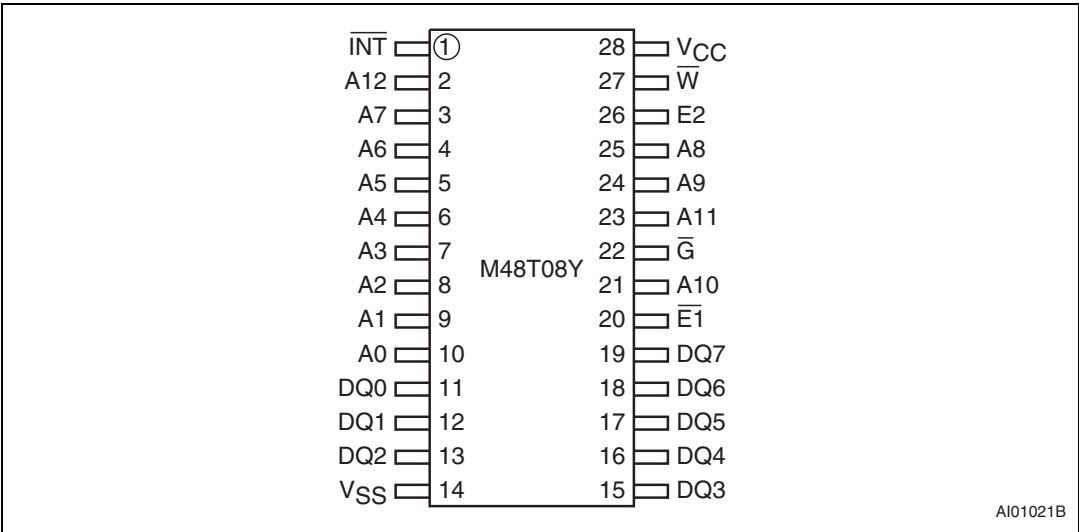
Figure 3. SOIC connections
